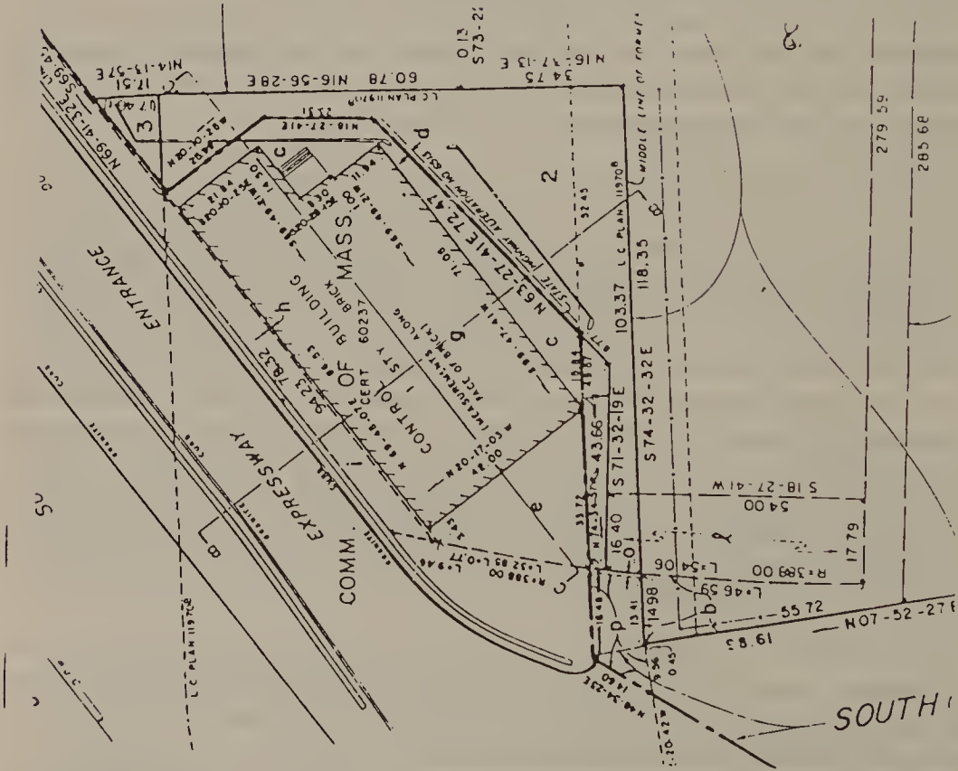
Fig. 5.4 Title insurance plan with certification by private land surveyor (from Greulich 1983)
