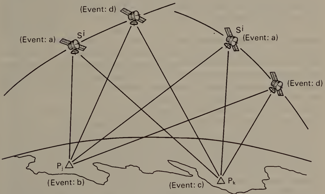
Fig. 9.1 GPS relative positioning (Wild Heerbrugg)
