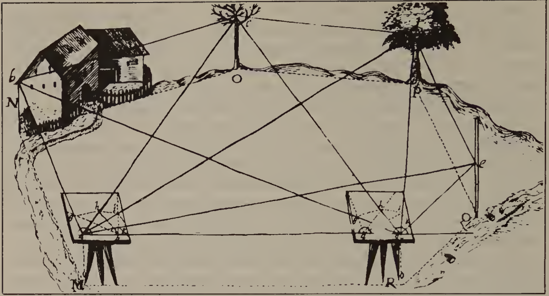
Fig. 9.2 Plane table (from Zubler 1601). It allows the map making in the open fields on the base of proportional triangles. All points are the points of intersection of the directions observed from the terminals of a base. The scale of the map results from the plotted length of the base. The maps produced were predominantly in scales of 1:1000, 1:2500, and 1:5000. A characteristic common to these surveys was that plane table positions were not monumented. Although the method results in relatively large uncertainties, experienced surveyors were able to achieve a graphical accuracy (within the range of scales mentioned) of \pm 20 cm to \pm 80 cm. Even today the plane table method can be cheap and efficient. It has the great advantage of permitting continuous comparison in the field between the actual topography and its plotted depiction.
