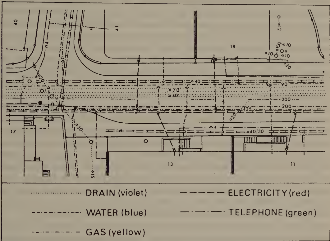
Fig. 4.4 Utility map, showing underground services (from Dale 1976)
